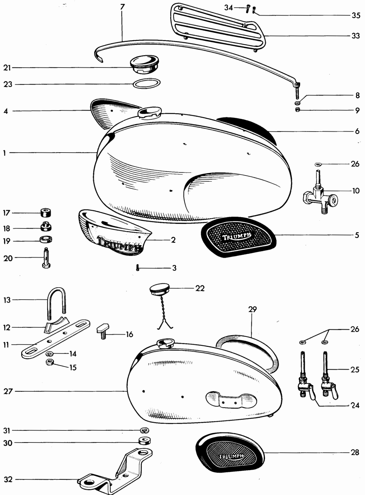
Fig. 25. PETROL TANK
